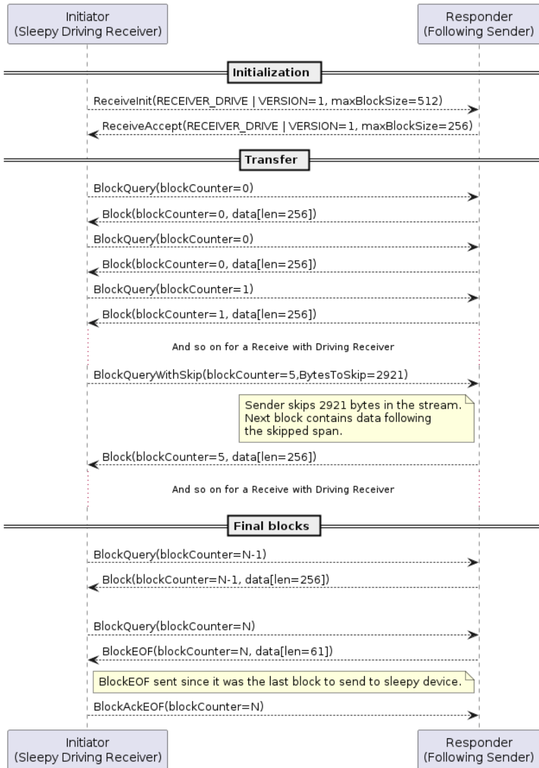
Figure 90. Synchronous file receiving by device acting as driving Receiver, including BlockQueryWithSkip
