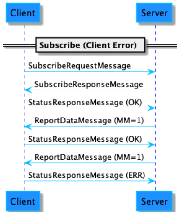
Figure 83. Subscription with client-side error flow
