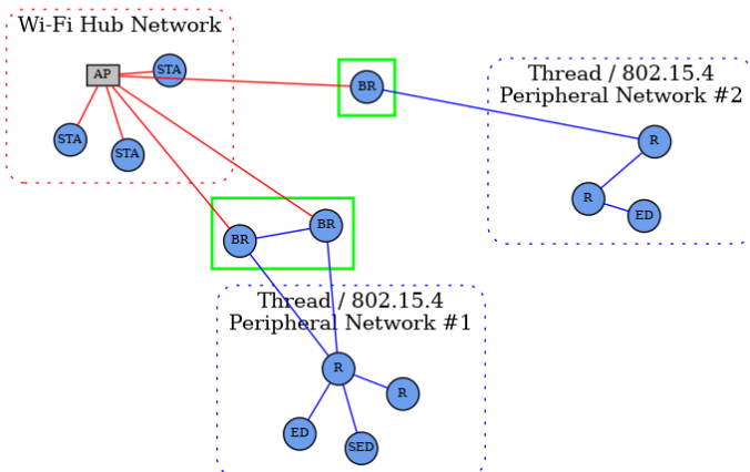
Figure 5. Star network topology
