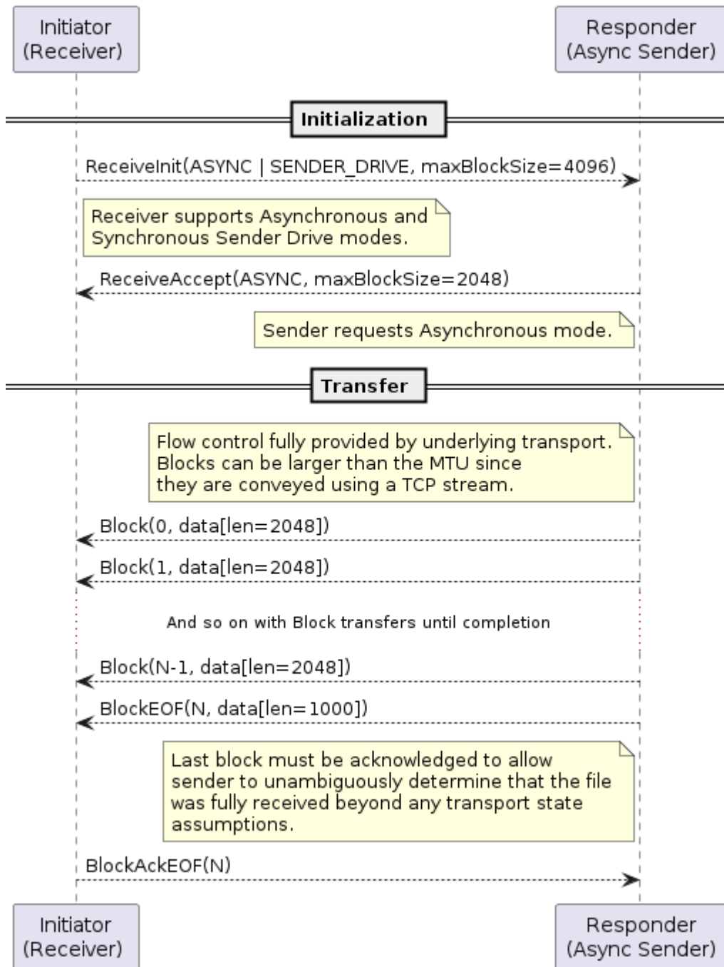
Figure 95. Asynchronous file receiving
