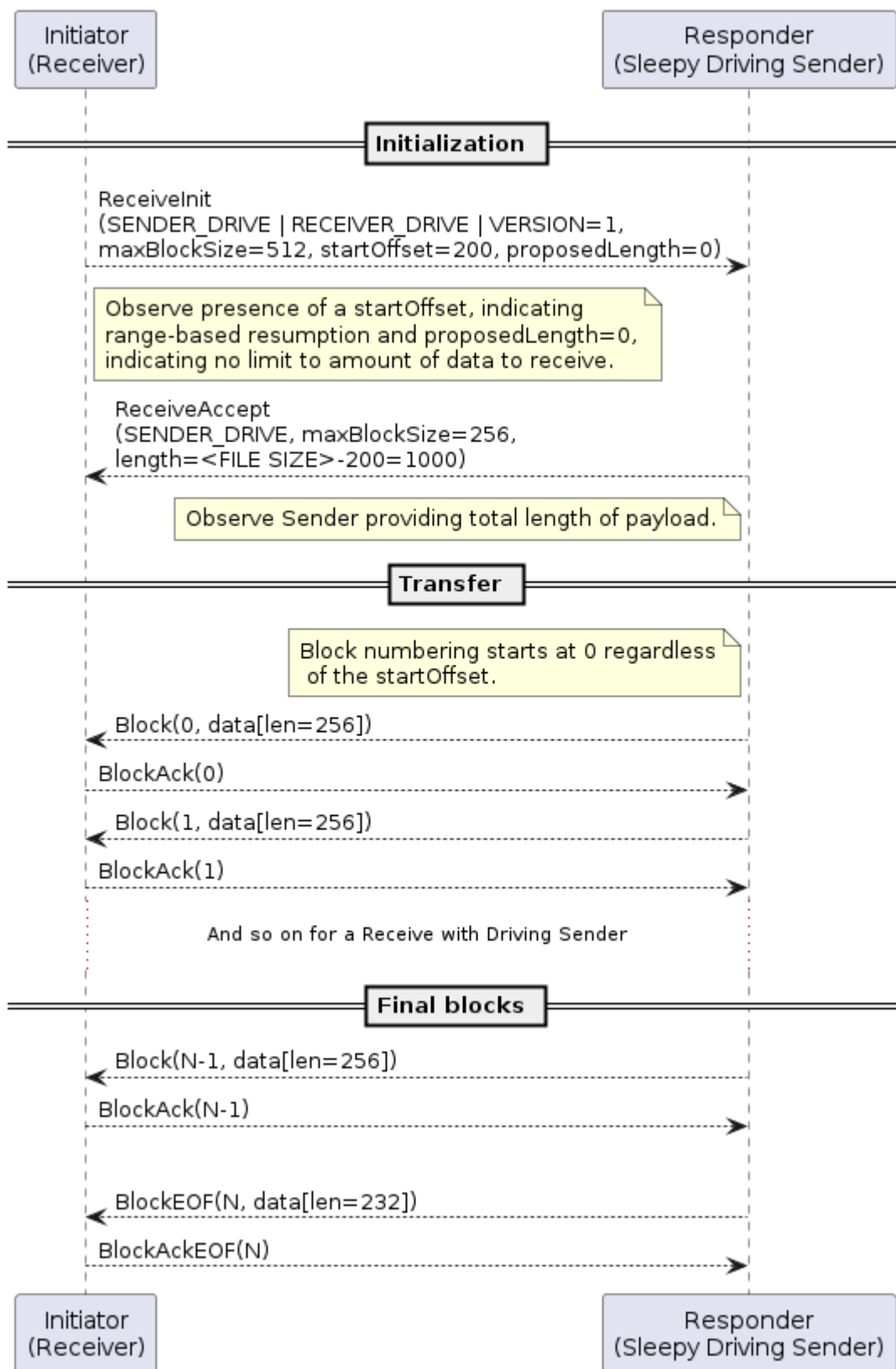
Figure 92. Re-started receive from sleepy device acting as driving Sender
