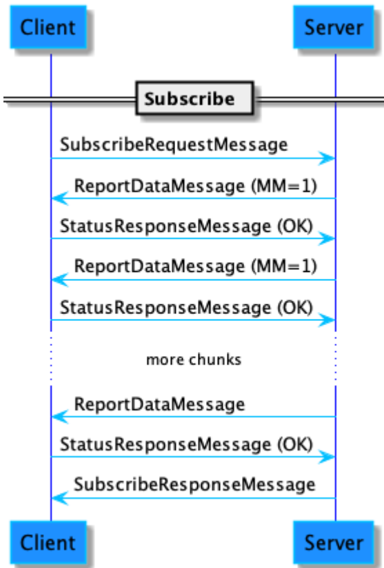
Figure 81. Subscription flow
