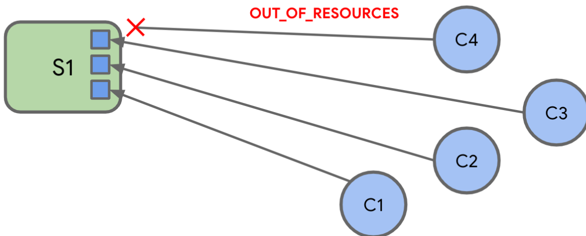
Figure 62. Rejection
