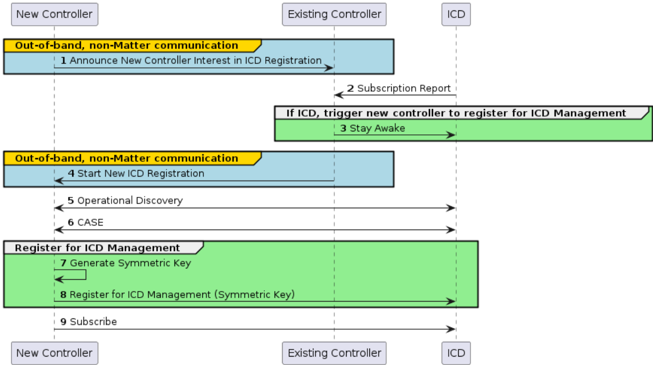
Figure 74. Infrastructure Assisted On-Demand Registration
