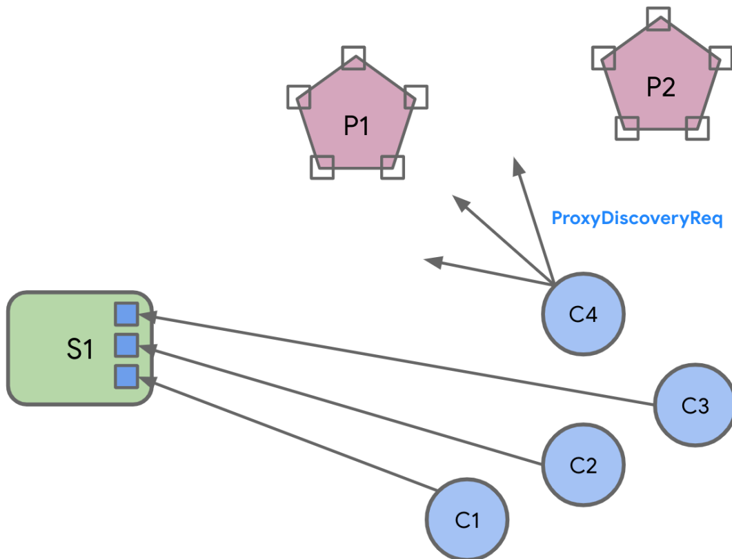
Figure 63. Discovery Request
