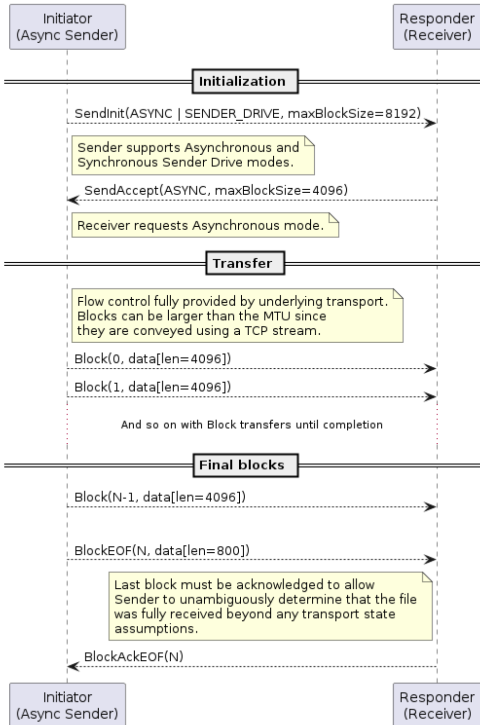
Figure 94. Asynchronous file sending
