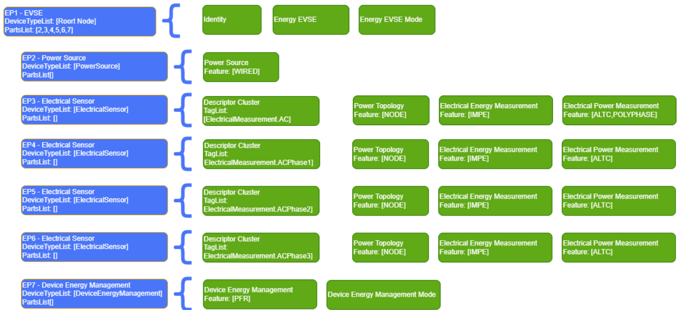
Figure 9. Example of a 3 phase EVSE
