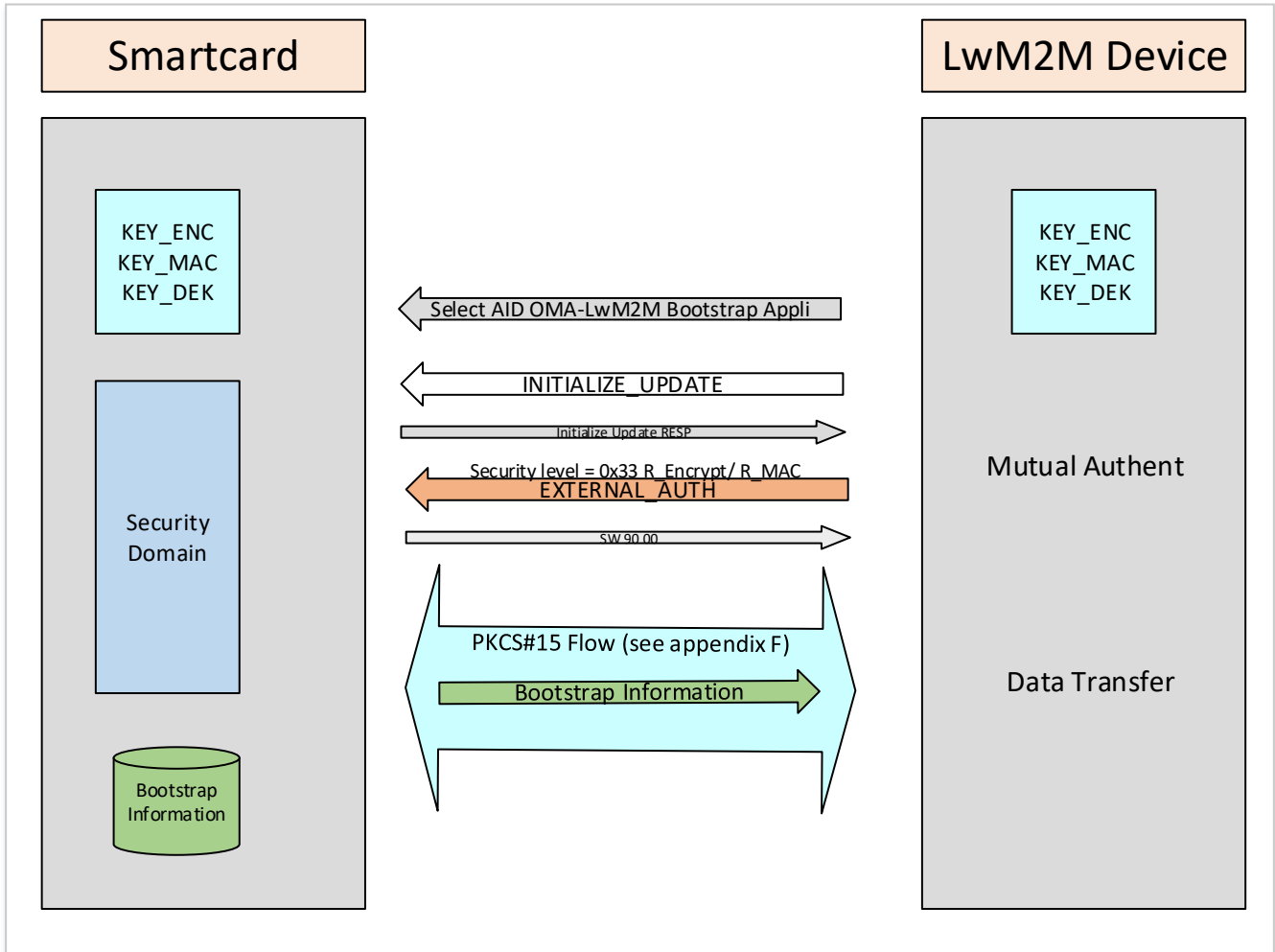
Figure 33: Bootstrap Information transfer from Smartcard to LwM2M Device using Secure channel according to [GLOBALPLATFORM] [GP SCP03] [GP AMD_A]
