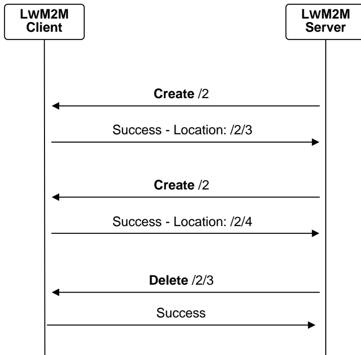
Figure 12: Example flows of Device Management & Service Enablement Interface
