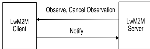
Figure 6: Information Reporting
