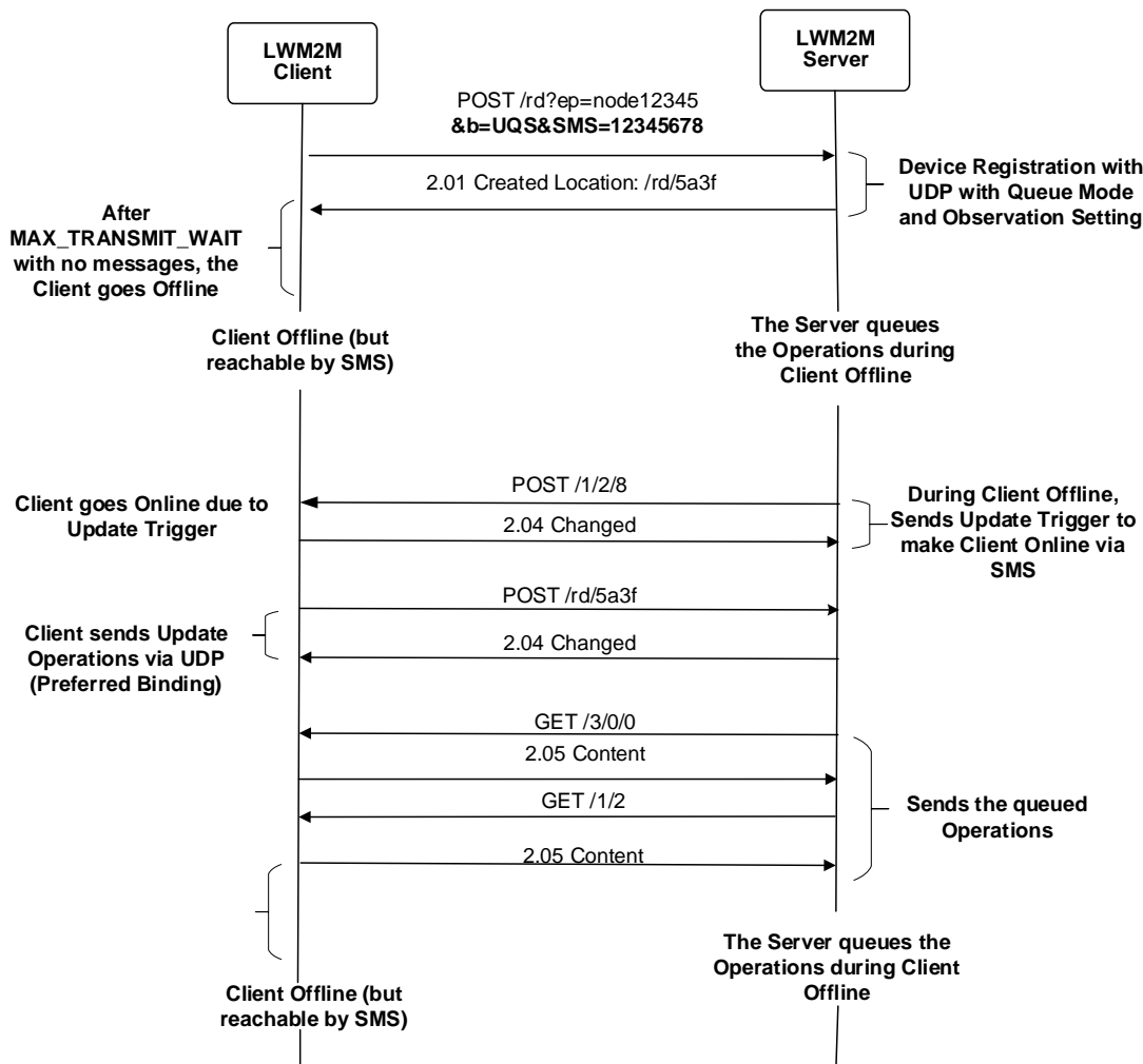
Example of Device Management & Service Enablement interface exchanges for Queue Mode with SMS Registration Update Trigger
