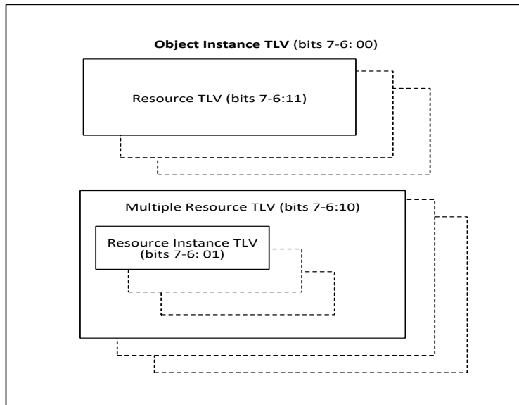
Figure 17: TLV nesting
