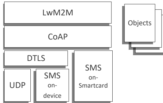
Figure 2: The protocol stack of the LwM2M Enabler.
