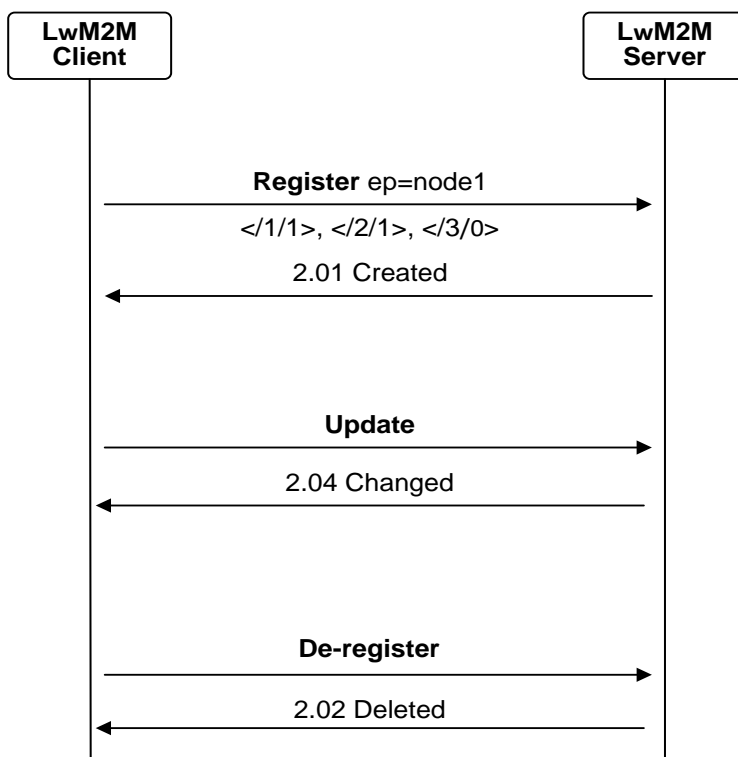
Figure 9: Client Registration Interface example flows
