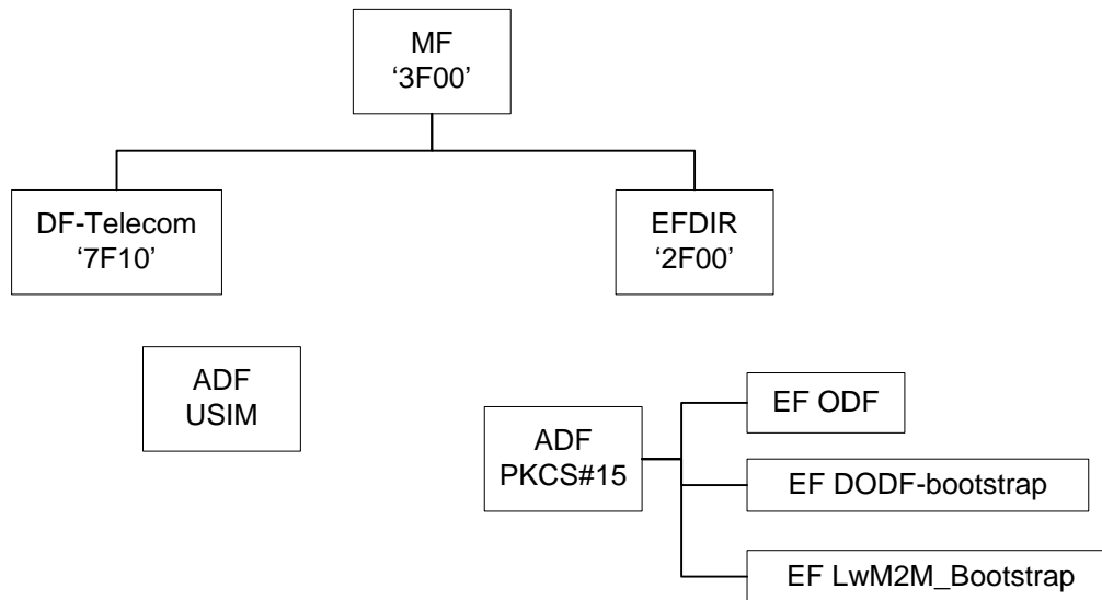
Figure 32: Example of a 3G UICC File Structure embedding a specific PKCS#15 file structure containing LwM2M Bootstrap data location
